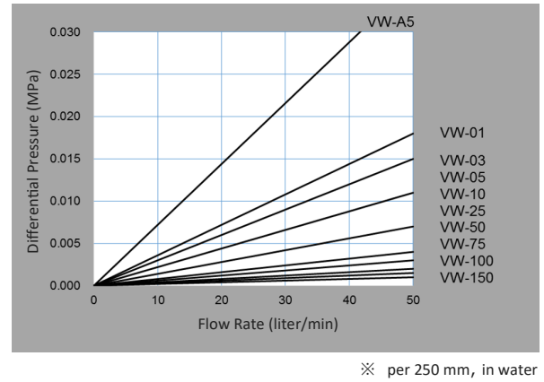
Flow Rate - Differential Pressure
